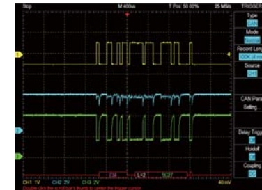
Decode the differential CAN signals with a differential probe. (CH1: Differential Probe, CH2: CAN H, CH3: CAN L)
